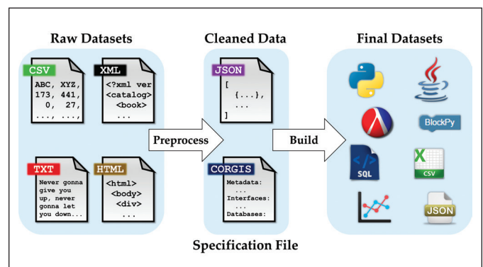
Figure 1: How datasets are added to CORGIS
