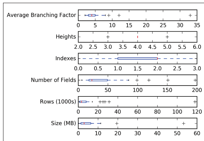
Figure 6: Distribution of structure and characteristics of CORGIS datasets
