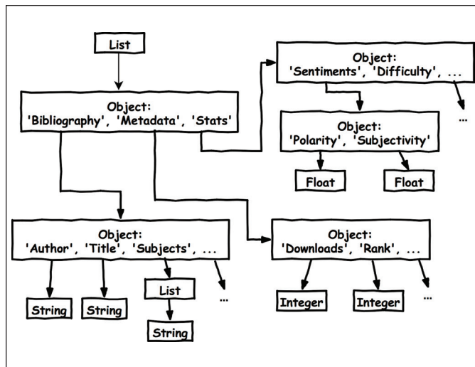
Figure 2: Partial data map for the Classics library
