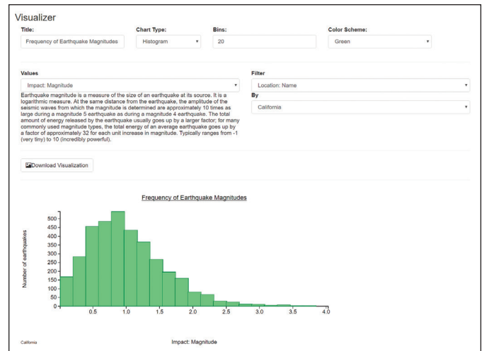
Figure 4: The CORGIS Visualizer
